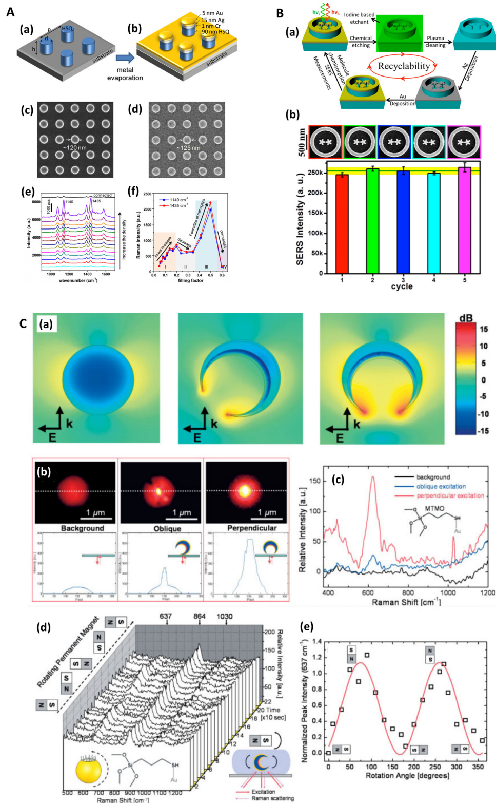
Fig. 8 Fill factor, reusability, and orientation. A. The effect of nanostructure density/fill factor on SERS (a) Schematics of electron beam lithography (EBL)-defined hydrogen silsesquioxane (HSiQ) nanoposts with diameter d and pitch p . (b) Schematics of the plasmonic nanostructures after depositing metal on HSiQ nanoposts. (c) SEM image of HSiQ nanoposts with a diameter of 120 nm and pitch of 240 nm. (d) SEM image of the plasmonic nanostructure array after metal deposition on HSiQ nanoposts in (c). (e) Raman scattering spectra of plasmonic nanostructures with varied density. (f) The SERS intensity as a function of the particle density. Reprinted with permission from Wei (2016) © The Optical Society. 104 B. Recyclable, ring-cavity-enclosed, bimetallic nanostars for SERS. (a) Illustration of the maskless recycling process that can be applied to 3D geometries such as AgAu-3D-nanostar-dimer-in-ring nanostructures. (b) SERS intensity of the p -aminothiophenol (pATP) band at 1077\text{ cm}^{-1} recorded after each recycling
