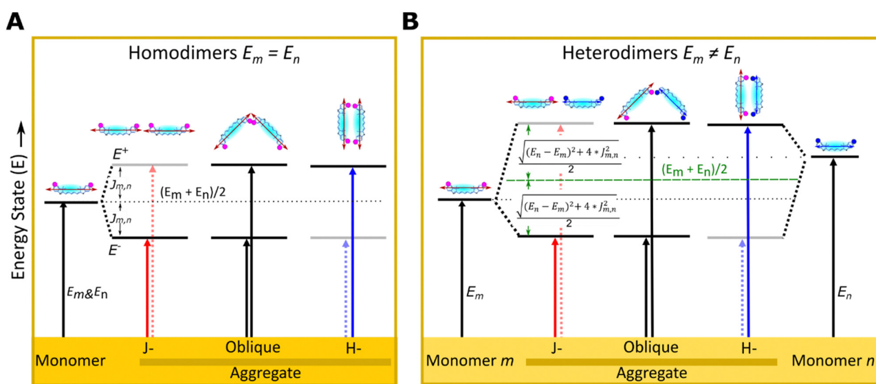
Fig. 1 Schematic illustration of electronic transitions of (A) homodimer ( m = n ) and (B) heterodimers ( m \neq n ) relative to their monomers m and n as described by molecular exciton theory. 34 The formation of dye aggregates induces exciton delocalization splitting into higher and lower excited energy states ( E^+ and E^- ) relative to the corresponding monomers. The transition into a higher- (lower-) energy excitonic state is forbidden for J- (H-) aggregates, respectively (dot arrows). In the dye structure, dots (purple and blue) represent modified substituents of Cy5-R in 5 and 5' positions of indole rings and the arrow represents the TDM orientation.
