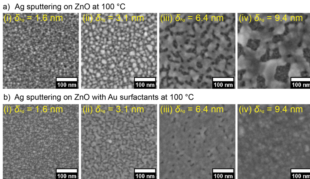
Fig. 6 FESEM images of sputter-deposited UTSLs at 100 °C on (a) the bare ZnO support and (b) the ZnO support with Au surfactant at different thicknesses of the UTSL \delta_{Ag} = 1.6, 3.1, 6.4 , and 9.4 nm, respectively.
