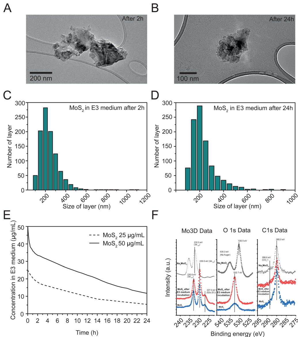
Fig. 1 Characterization of exfoliated \text{MoS}_2 . (A) HRTEM images after 2 hours and (B) 24 hours and corresponding layer size distributions in E3 medium after 2 hours (C) and 24 hours (D). (E) Colloidal stability of \text{MoS}_2 in zebrafish E3 medium at 25 and 50 \mu\text{g mL}^{-1} during 24 h. (F) Signals from XPS analyses before (blue traces) and after 24 hours exposure to E3 medium (red traces). Molybdate salt (black traces) was used as reference control.
