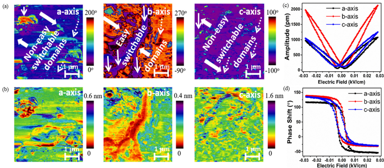
Fig. 2 (a) Vertical PFM phase images recorded on a single crystal of 1 oriented along a -, b - and c -axis and (b) corresponding amplitude images showing the different domains, (c) amplitude vs. electric field butterfly loop, (d) phase shift vs. electric field hysteresis loop along the three directions (applied voltage is normalized with respect to electric field).
