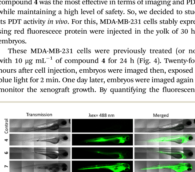
Fig. 3 Casper zebrafish embryos at 72 hours post-fertilization (hpf) were injected with 10 nL of 4 , 6 , 7 at a concentration of 1 mg mL -1 in 5% glucose (final concentration \sim 111 \mu\text{g mL}^{-1} ). Embryos injected with 4 and 6 were observed with LSM880 (laser power 30%) 3 h post-injection. Embryos injected with 7 were observed with LSM880 (laser power 1%) immediately after injection.
