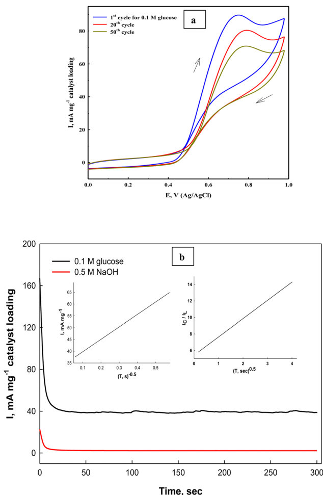
Fig. 12 (a) Repeated cyclization of the Ni(II)-SB/C electrode in 0.5 M NaOH + 0.1 M glucose, and (b) chronoamperometry of the same electrode at 0.72 V and the inset plots represent I and 1/\text{square root of time} (left) and the relationship of I_C/I_L and square root of time (right).
