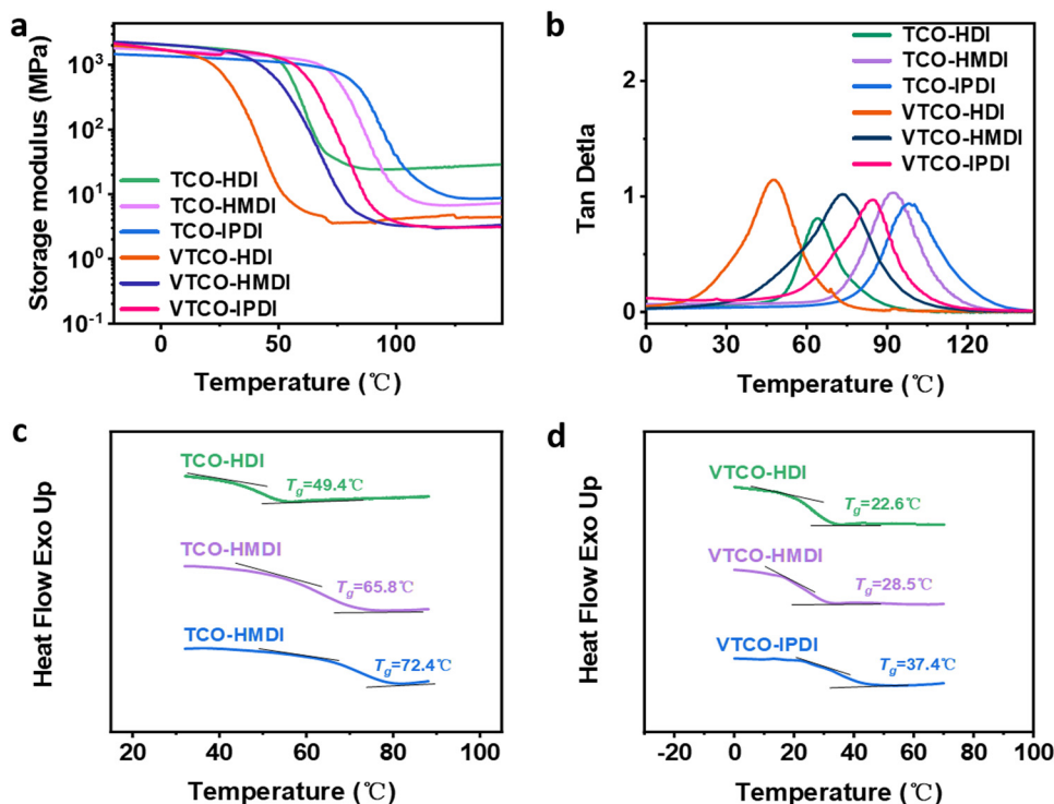
Fig. 3 (a) Storage modulus and (b) tan \delta as a function of temperature for TCO-NCO and VTCHCO by DMA. (c) DSC curve of TCO-NCO. (d) DSC curve of VTCHCO.
