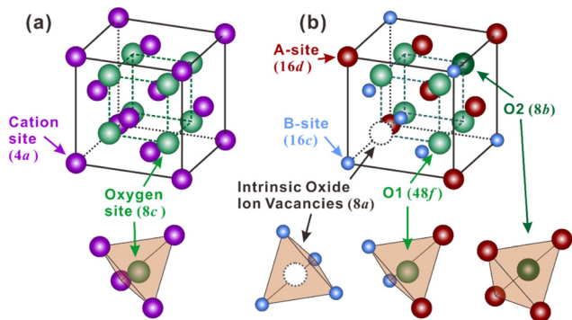
Fig. 1 (a) Fluorite and (b) pyrochlore crystal structures.
