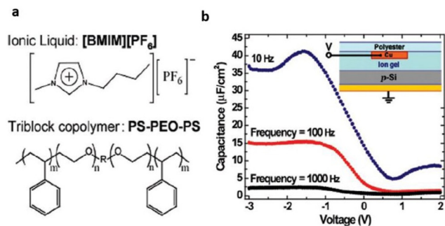
Fig. 7 (a) Structure of the ionic liquid and triblock copolymer ion gel components (b) C-V characteristics of a p\text{-Si}/\text{ion gel}/\text{Cu} test structure (see inset) at three frequencies (right). The C-V curves indicate large frequency-dependent hole accumulation in the Si at negative bias on the top contact. Reproduced from ref. 71 with permission from ACS, Copyright [2007].
