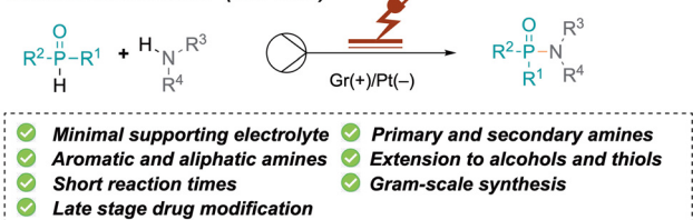
Scheme 1 Challenges and benefits of previous synthetic approaches and current work.
