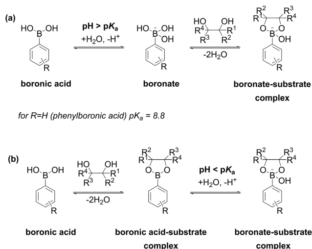
Fig. 4 Two modes of complexation via (a) ionization of the boronic acid and (b) its direct complexation with a diol.
