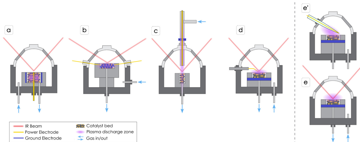
Fig. 2 Schematic of operando DRIFTS configurations developed by research groups for investigating plasma catalysis under reaction conditions. (a) DBD embedded within the catalyst bed, (b) helical surface DBD, (c) DBD above the catalyst bed, (d) point-source DBD, (e) and (e') point-source DBD with two different views (this study). The dielectric is: (a) the quartz capillary covering the power electrode, (b) a coating on the power electrode, (c) the quartz tube containing the plasma discharge zone, (d) the sample holder depicted in light grey, (e) and (e') the quartz tube covering the power electrode tip.
