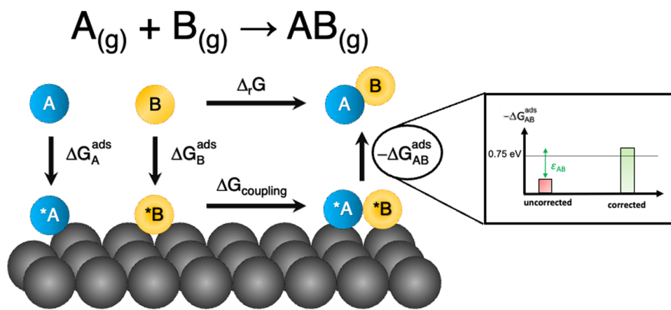
Fig. 9 Scheme of a catalytic coupling reaction. Inset: Desorption energy of AB before (in red) and after (in green) correcting gas-phase errors. In the example, without gas-phase errors, easy desorption is predicted, whereas site blocking is predicted upon incorporating them. Adapted from ref. 25 Copyright 2021, John Wiley and Sons.
