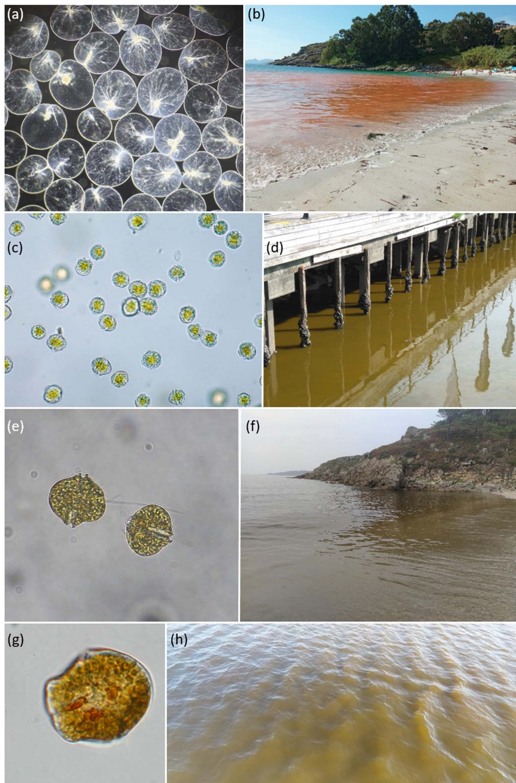
Fig. 6 Images of selected red tides and responsible species in Galicia. Microscopic images not to scale: (a) N. scintillans , (b) red tide of N. scintillans (Areaimilla, Cangas, 2021), (c) A. minutum , (d) red tide of A. minutum (Vigo, 2018; author: M. Garci), (e) A. tamarense , (f) red tide of A. tamarense (Rebordelo, 2021; author: A. Fuentes), (g) K. triquetrum (author: R. Figueroa), and (h) red tide of K. triquetrum (Nigrán, 2023; author: G. González-Nuevo).
