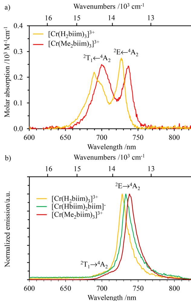
Fig. 4 NIR (a) absorption spectra of [\text{Cr}(\text{H}_2\text{biim})_3](\text{NO}_3)_3 (water) and [\text{Cr}(\text{Me}_2\text{biim})_3](\text{CF}_3\text{SO}_3)_3 (acetonitrile) and (b) emission ( \lambda_{\text{exc}} = 330 \text{ nm} ) spectra of complexes [\text{Cr}(\text{H}_2\text{biim})_3](\text{NO}_3)_3 (orange), [\text{Cr}(\text{Hbiim})_2(\text{biim})]^- \text{PPh}_4 (green) and [\text{Cr}(\text{Me}_2\text{biim})_3](\text{CF}_3\text{SO}_3)_3 (red) in MeOH at 293 K.
