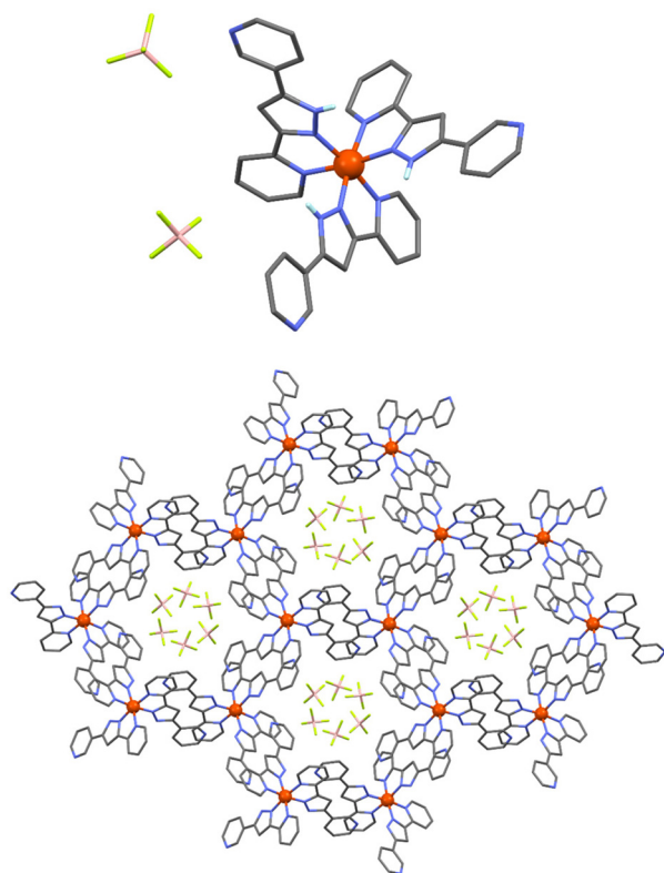
Fig. 1 Representation of [\text{Fe}(\text{HL})_3](\text{BF}_4)_2 ( 1 ) (top) and the crystal packing along the c axis (bottom). Fe, N, C, B, F and H atoms are shown in orange, blue, grey, pink, green and white, respectively. Only H atoms from the pyrazolyl NH groups are shown for clarity.
