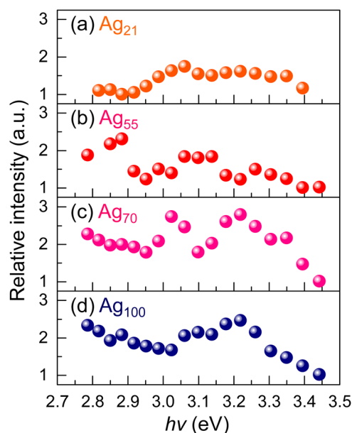
Fig. 5 Photon energy dependence of photoemission in Ag_n/C_{60} ( n = 21, 55, 70 , and 100 ), measured with s -polarized light within the range of 2.77 to 3.45 eV. Above n = 70 , photoemission enhancements with s -polarized light are observed, resulting in a decrease in I_p/I_s values.
