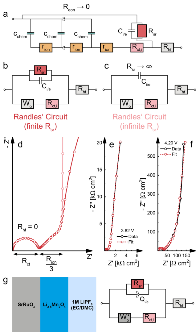
Fig. 9 (a) Simplified transmission line for a dense Li insertion electrode with \sigma_{ion} \ll \sigma_{eon} ( R_{eon} \approx 0 ). The electronic rail is replaced by a short circuit, allowing the replacement of the transmission line by a W_o element. A high-frequency offset resistance R_{hf} has been added in series to account for ohmic impedance contributions from the electrolyte and other cell components. (b) Randles' circuit with a finite R_{sr} in parallel to C_{i/e} . (c) Classical Randles' circuit, assuming an infinite R_{sr} . (d) Calculated impedance responses of the circuits from subfigures (b) and (c), where R_{hf} has been neglected in both cases. (e) Half-cell impedance spectra of an LMO thin film electrode at 3.82 V versus Li (low C_{chem} ). Diagram reproduced with data from ref. 5. (f) Half-cell impedance spectra of an LMO thin film electrode at 4.20 V versus Li (high C_{chem} ). Diagram reproduced with data from ref. 5. (g) Sample sketch and equivalent circuit used for fitting the impedance spectra (e) and (f).
