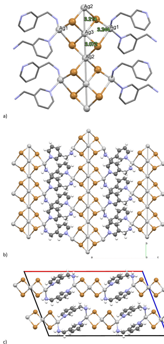
Fig. 2 (a) Inorganic saddle chain; (b) 2-D network with the inorganic chain parallel to the b -axis and (c) packing along the b -axis of [(\text{AgBr})_2(3\text{-pica})]_n . Cell axis color: a is red, b is green, and c is blue.
