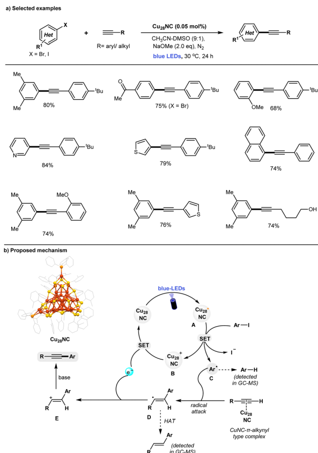
Fig. 3 Defects \text{Cu}_{28}\text{NC} catalyzed Sonogashira C-C coupling reactions under photoinduced conditions.
