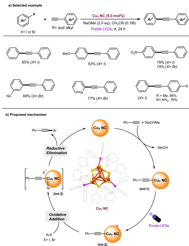
Fig. 4 Luminescent \text{Cu}_7\text{NC} catalyzed Sonogashira C-C coupling reactions under photoinduced conditions.
