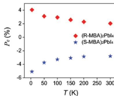
Fig. 8 Temperature-dependent CPL for (R/S\text{-MBA})_2\text{PbI}_4 . Reprinted with permission from ref. 27 Copyright©2022 Royal Society of Chemistry.
