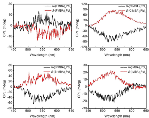
Fig. 7 CPL spectra of (R/S\text{-}4\text{-X-MBA})_2\text{PbI}_4 , X = F, Cl, Br, I. Reprinted with permission from ref. 26 Copyright©2021 Wiley-VCH GmbH.
