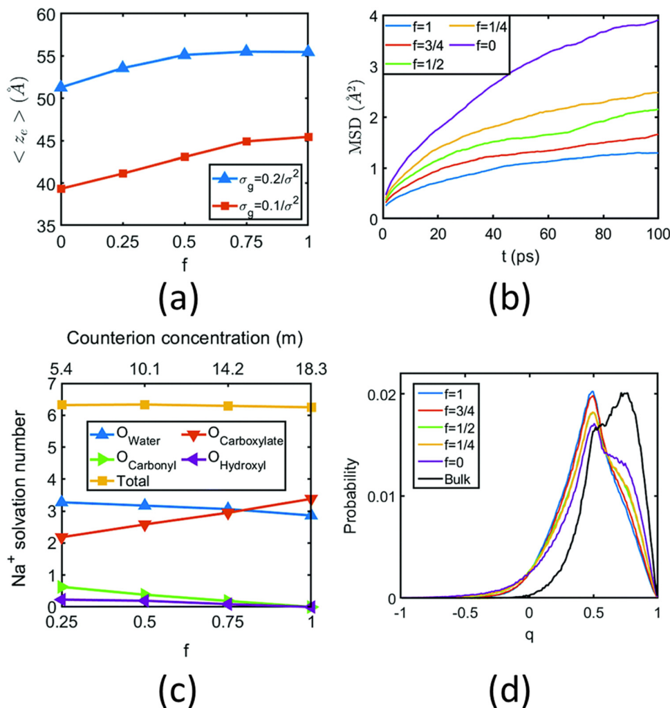
Fig. 11 (a) Variation of the height ( \langle z_e \rangle ) of the \text{Na}^+ -counterion-screened PAA PE brushes with degree of ionization ( f ) for two different values of the PE brush grafting density. (b) MSD of the backbone carbon atoms of the PAA PE brushes for different degrees of ionization of the PAA brushes for a grafting density ( \sigma_g ) of 0.1/\sigma^2 chains per \text{nm}^2 ( \sigma = 3.5 Å). (c) Change in the composition of the solvation shell of the brush-supported \text{Na}^+ counterions with the degree of ionization of the PAA brushes (for \sigma_g = 0.1/\sigma^2 chains per \text{nm}^2 ). (d) Variation in the probability of the tetrahedral order parameter ( q ) of the water molecules with the degree of ionization ( f ) of the PAA brushes (for \sigma_g = 0.1/\sigma^2 chains per \text{nm}^2 ). All the parts of the figure have been reproduced from Sachar, H. S.; Pial, T. H.; Chava, B. S.; Das, S., All-atom molecular dynamics simulations of weak polyionic brushes: influence of charge density on the properties of polyelectrolyte chains, brush-supported counterions, and water molecules, Soft Matter , 2020, 16 (33), 7808–7822. Copyright (2020) Royal Society of Chemistry (UK).
