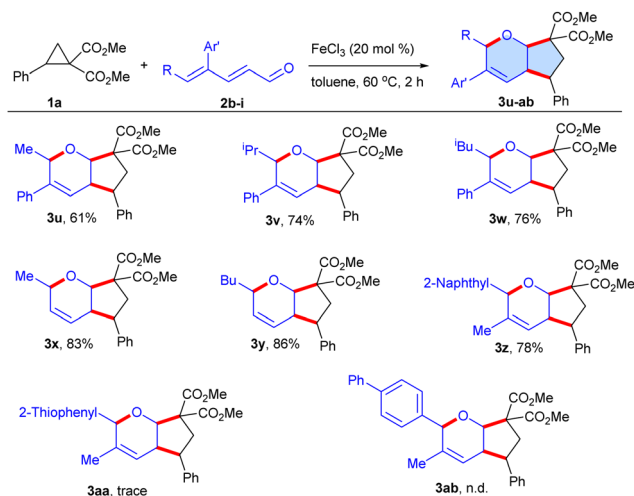
Scheme 5 Preliminary mechanistic investigation.
