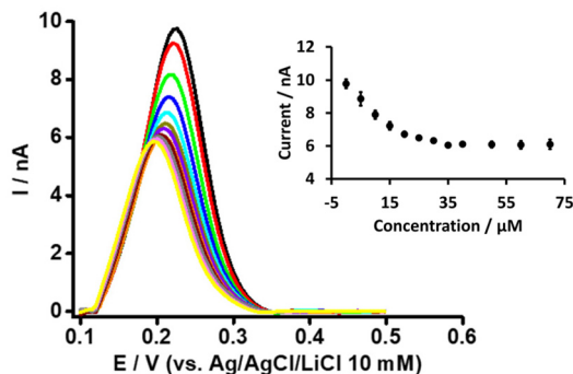
Fig. 4 DPVs at different concentrations of \beta -CD at a fixed concentration of PFOA (5 \mu M) at the \mu ITIES array. Cell composition as shown in Scheme 1. Black, red, green, blue, cyan, dark yellow, violet, orange, wine red, gray, magenta, and yellow, respectively, represent the DPVs at 0, 5, 10, 15, 20, 25, 30, 35, 40, 50, 60, and 70 \mu M \beta -CD. Inset: relationship between current and concentration of \beta -CD. DPVs are background-subtracted followed by baseline-corrected. Error bars indicate \pm 1 standard deviation from three independent measurements.
