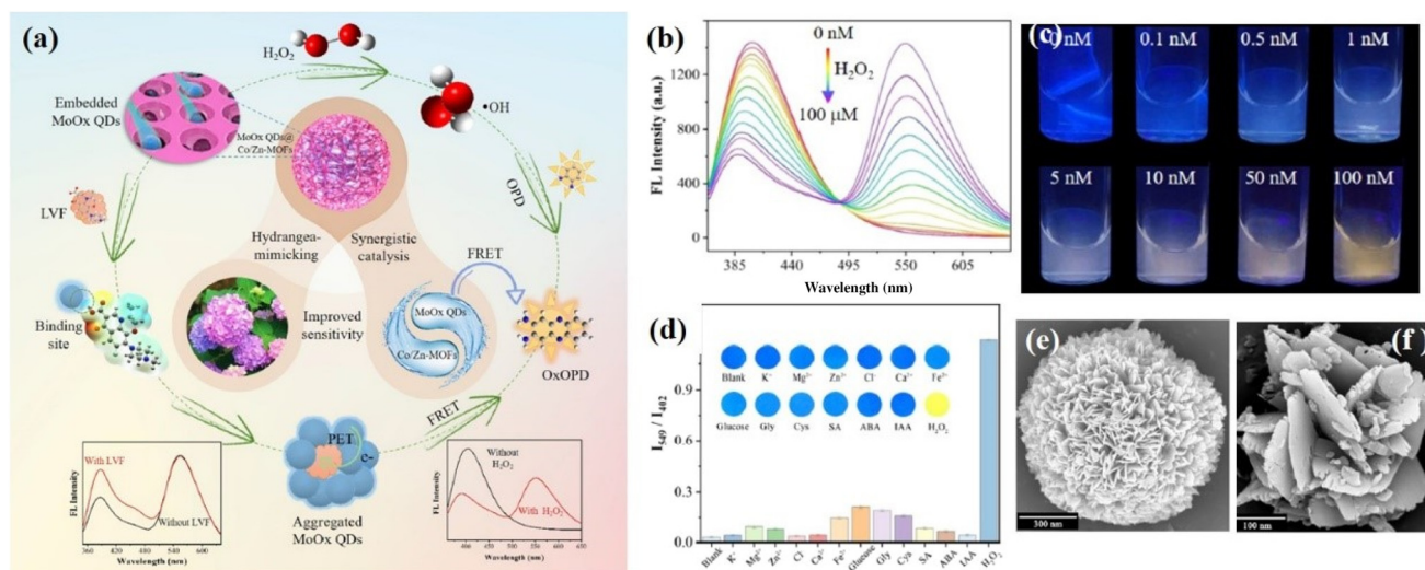
Fig. 21 (a) A schematic diagram of MoOx QDs@Co/Zn-MOFs for the detection of \text{H}_2\text{O}_2 and LVF. (b) The fluorescence spectra of the probe exposed to different concentrations of \text{H}_2\text{O}_2 and (c) solution under ultraviolet light with a catalytic reaction, (d) was the selectivity experiment. The SEM image of MoOx QDs@Co/Zn-MOFs before (e) and after (f) reaction with \text{H}_2\text{O}_2 for 1.0 h. Reproduced with permission from ref. 334. Copyright 2022, Elsevier.
