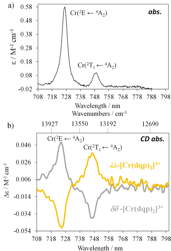
Fig. 2 (a) Absorption spectrum of the rac-[Cr(dqp)_2]^{3+} and (b) CD spectra in the spin-flip region for the two enantiomers ( \text{CH}_3\text{CN} ; c = 1 \text{ mM} ).
