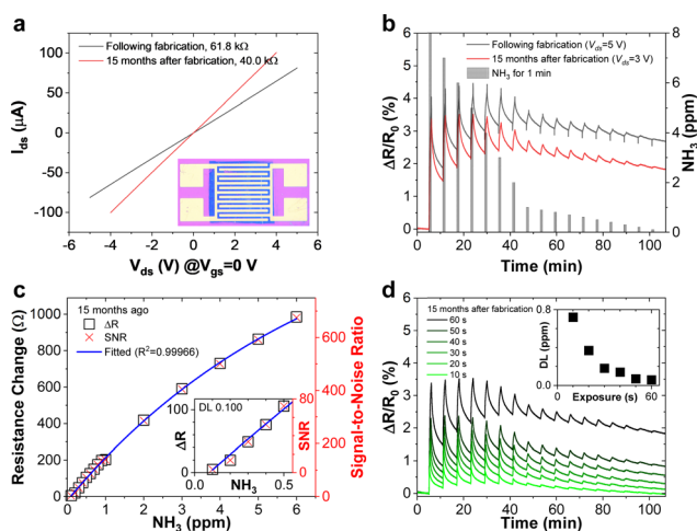
Fig. 3 (a) Current–voltage ( I_{\text{ds}}-V_{\text{ds}} ) characteristics of an LPE-PtSe 2 LB film sensor showing a noticeable conductance change after long-term exposure to the atmosphere. Inset: photograph of an LPE-PtSe 2 LB film (blue area) underneath interdigitated electrodes. (b) Sensor response curves of the LPE-PtSe 2 LB film sensor upon introduction of periodically decreasing concentrations of NH 3 from 8 down to 0.1 ppm (gray columns) at room temperature. A NH 3 sensor response is still observed 15 months later. (c) Resistance (open boxes) and SNR (red x-crosses) changes are proportional to the introduced gas concentration. Inset: zoomed-in plot in the lower NH 3 concentration range. (d) Sensor response curves for 10 to 60 seconds of NH 3 gas introduction (from light green to dark green). Inset: detectable NH 3 gas concentration inversely decreases as the gas exposure time increases.
