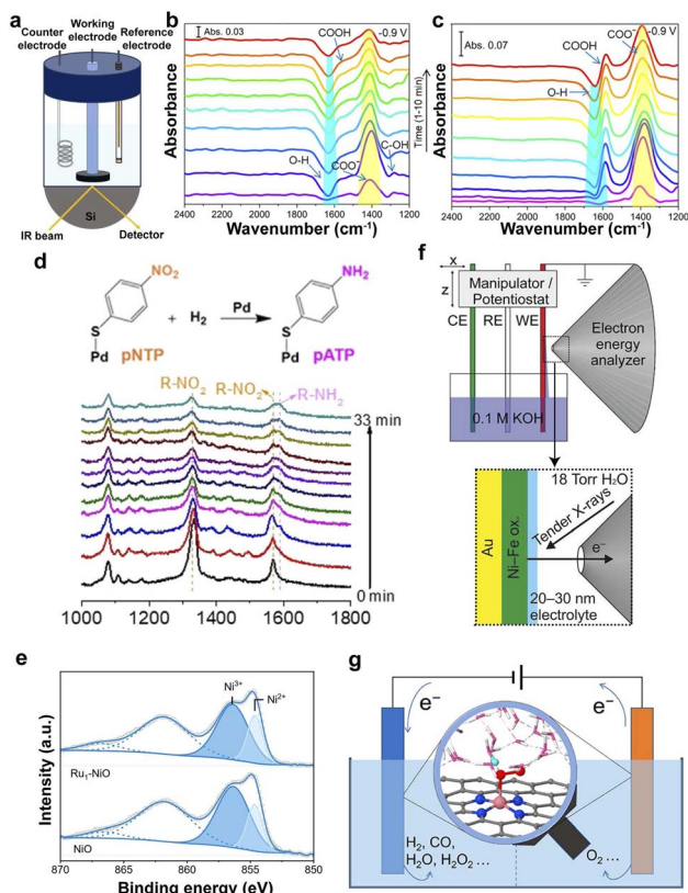
Fig. 3 (a) Schematic illustration of the in situ FT-IR configuration for the \text{CO}_2 RR. Time-dependent in situ IR spectra taken at -0.9 V (vs. RHE) in the \text{CO}_2 RR conditions on \text{PdIn@In}_2\text{O}_3 (b) and PdIn alloy (c) during the second chronoamperometric test at -0.9 V. 121 Copyright 2022, American Chemical Society. (d) Diagram and in situ SERS of the hydrogenation of pNTP over Pd SACs under \text{H}_2 at 80^\circ\text{C} . 127 Copyright 2021, Wiley. (e) XPS in the Ni 2p region for NiO and \text{Ru}_1\text{-NiO} . 129 Copyright 2022, Wiley. (f) Schematic illustration of an electrochemical cell. 130 Copyright 2016, American Chemical Society. (g) Understanding electrocatalysis at SACs from simulations under realistic electrochemical environments. 135 Copyright 2022, American Chemical Society.
