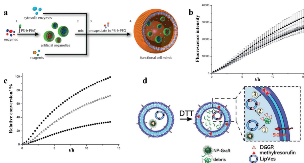
Fig. 13 (a) Schematic representation of polymersomes-in-polymersome microreactor. (b) Ensemble fluorescence measurements of the cascade reaction with all of the enzymes free in solution (▲), CalB in polystyrene- block -poly( L -isocycanoalanine (2-thiophen-3-ylethyl)amide) (PS- b -PIAT) nanoreactors (■), or CalB and ADH in PS- b -PIAT nanoreactors (○). (c) Ensemble fluorescence measurements of the cascade reaction with CalB in PS- b -PIAT nanoreactors (■), alcalase in PS- b -PIAT nanoreactors (Δ), free alcalase (●). Reprinted from ref. 106. Copyright 2014, Wiley-VCH. (d) The schematic representation of the enzymatic reaction of lipase substrate (DGGR) loaded on nano-particles and LipVes loaded with lipase enzyme, and these polymersomes are encapsulated as subcompartments into a polymer GUV. Reprinted from ref. 107. Copyright 2020, Wiley-VCH.
