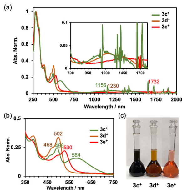
Fig. 4 (a) Absorption spectra of 3c^+ – 3e^+ in CH_2Cl_2 , (b) enlarged view of the spectra in the visible light range, and (c) photographs of the solutions ( [3c^+] – [3e^+] = 2.1 \times 10^{-5} M in CH_2Cl_2 ).
