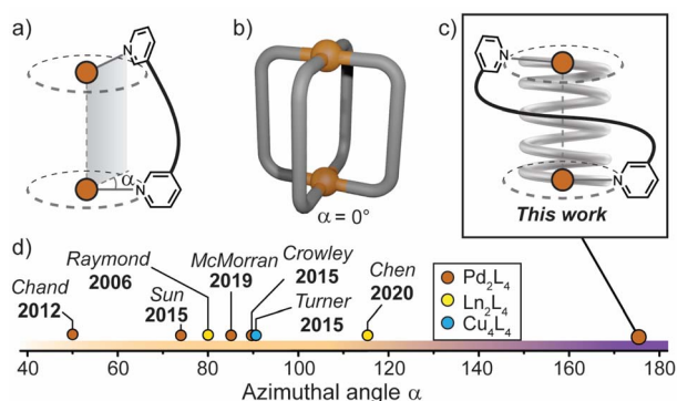
Fig. 1 (a) Azimuthal angle ( \alpha ) for a \text{M}_2\text{L}_4 helicate; (b) general structure of a non-helical \text{M}_2\text{L}_4 cage, where \alpha = 0^\circ ; (c) this work: a tightly-wrapped \text{Pd}_2\text{L}_4 helicate that behaves as a supramolecular spring; (d) azimuthal angles (extracted from X-ray diffraction data) of selected quadruple-stranded metallohelicates, shown for comparison. 15,39,42–46
