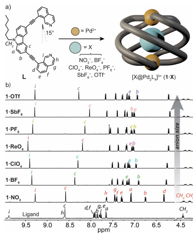
Fig. 2 (a) A scheme showing the structure and native bite angle of L and its self-assembly with \text{Pd}^{\text{II}} to give the \text{Pd}_2\text{L}_4 helicate 1 ·X, where X = different anionic guests; (b) ^1\text{H} NMR spectra (500 MHz/ \text{CD}_3\text{CN} ) of ligand L (bottom) and 1 ·X (top).
