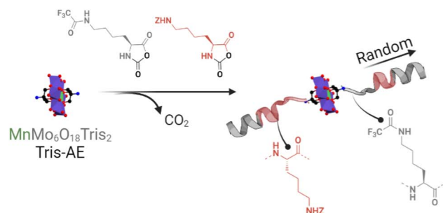
Fig. 10 (A) General scheme for the synthesis of POMlymers from random copolymers by the on-POM ring opening polymerisation (ROP) of NCAs – lysine trifluoroacetate NCA (grey, TFA K) and benzyloxycarbonyl lysine NCA (ZK NCA). (B) 1 H-NMR characterisation of POMK 30 TFA which stands for 30 TFAK residues.
