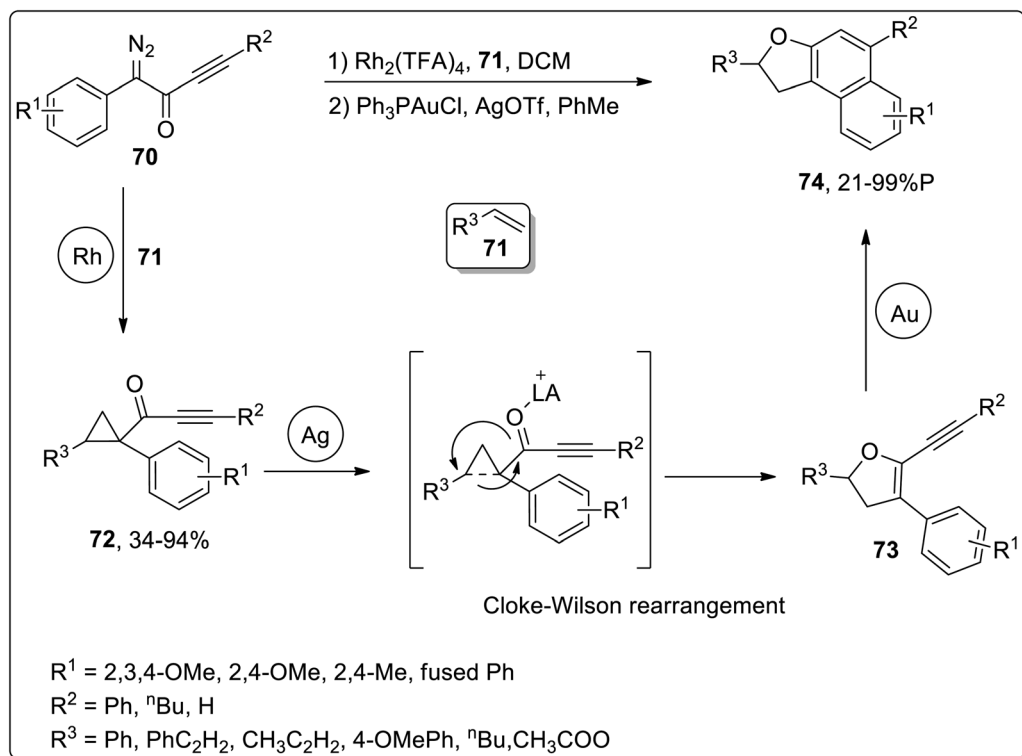
Scheme 23 Synthesis of benzo-fused dihydrofurans 74 via Cloke–Wilson rearrangement.
