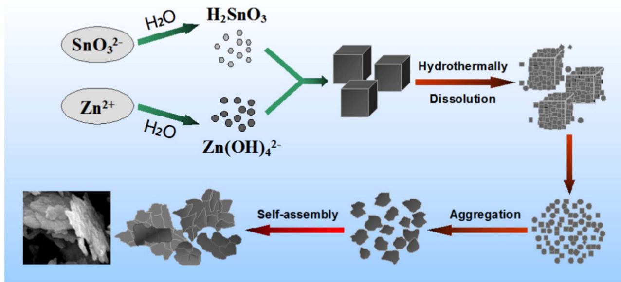
Fig. 10 Diagram depicting the probable process for the formation of the precursor \text{ZnSn}(\text{OH})_6 . 95
