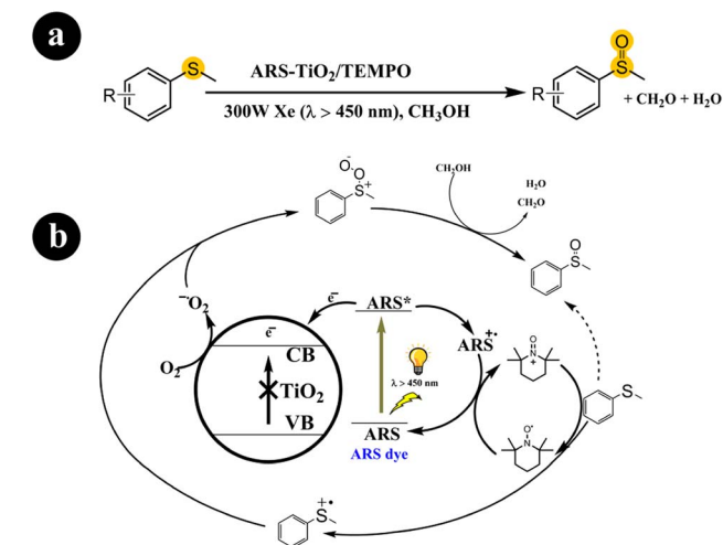
Scheme 5 (a) The reaction conditions for this process include specific parameters such as the type of catalyst (ARS-sensitized TiO 2 ), the presence of a co-catalyst (TEMPO), the use of visible light as the energy source, and the involvement of molecular oxygen (aerobic conditions). (b) One potential mechanistic route for the visible light photocatalytic aerobic oxidation of thioanisole involves ARS-sensitized TiO 2 and TEMPO. Reproduced with permission from ref. 40. Copyright 2016, John Wiley and Sons.
