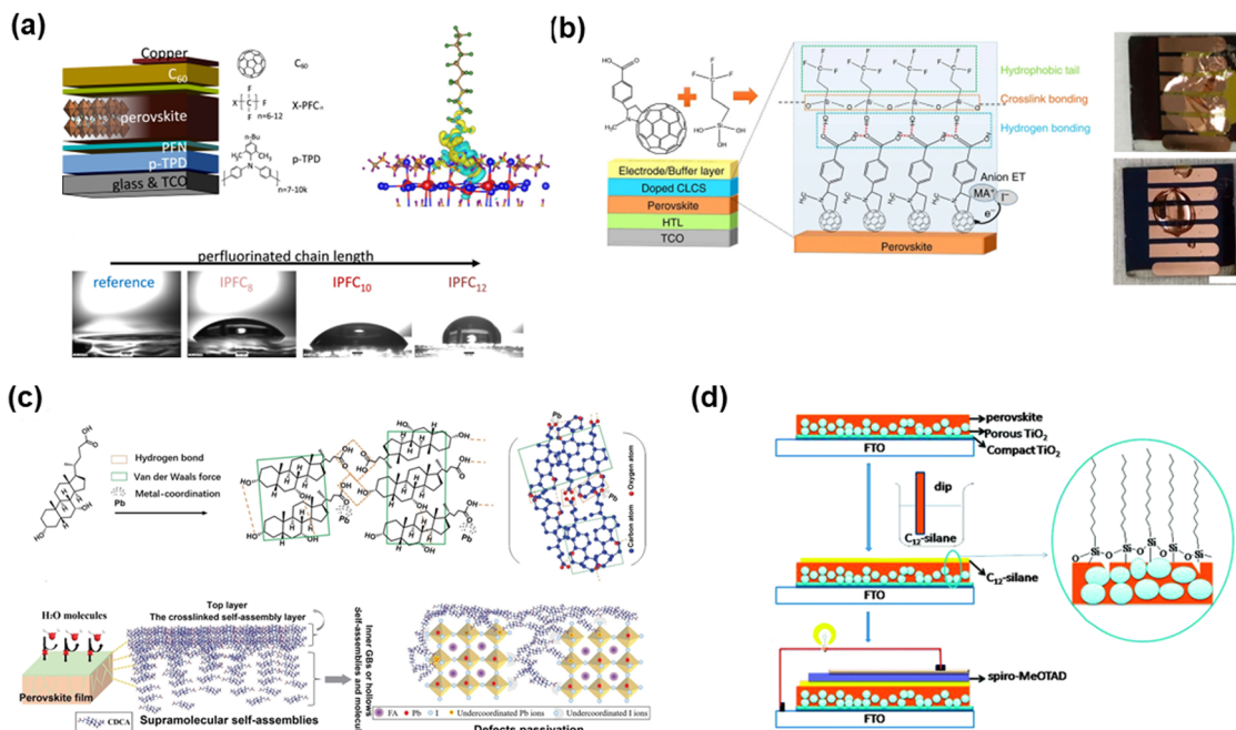
Fig. 18 SAMs on the top of perovskite film: (a) perfluorinated aliphatic carbon chains with iodine (X-PFC n ). Reproduced with permission. 111 Copyright 2020, the American Chemical Society. (b) Cross-linkable silane-functionalized fullerene SAMs. Reproduced with permission. 112 Copyright 2016, Nature. (c) Cholesterol derivative SAMs. Reproduced with permission. 113 Copyright 2022, Wiley-VCH Verlag GmbH & Co. KGaA, Weinheim. (d) C 12 -silane SAMs. Reproduced with permission. 114 Copyright 2015, The Royal Chemical Society.
