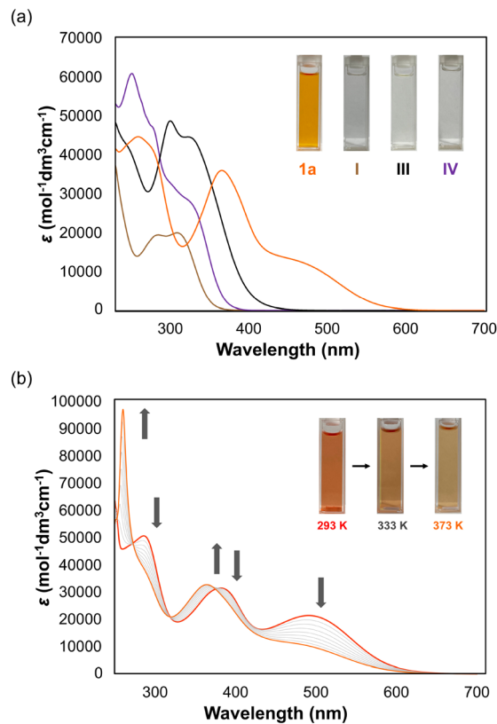
Fig. 2 (a) UV/Vis spectra of 1a , I , III , and IV in CH_2Cl_2 . (b) VT UV/Vis spectra of 1b in DMSO from 293 K to 373 K (every 10 K).
