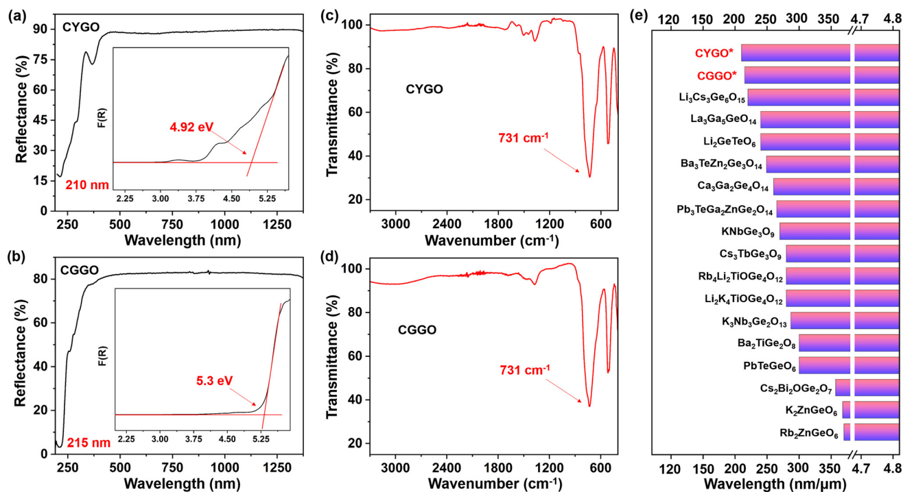
Fig. 3 (a and b) UV-vis-NIR diffuse reflectance spectra of the \text{CYGO} and \text{CGGO} , respectively; (c and d) IR spectrum of the \text{CYGO} and \text{CGGO} , respectively; (e) comparison of the UV cutoff edge among the boron-free germanate-based NLO crystals (* refers to compounds derived from this work).
