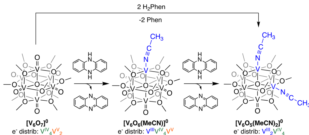
Scheme 1 Synthesis of O-atom vacancies in POV-alkoxide clusters via net H-atom uptake in MeCN; formation of [V_6O_6(\text{MeCN})]^0 and [V_6O_5(\text{MeCN})_2]^0 .
