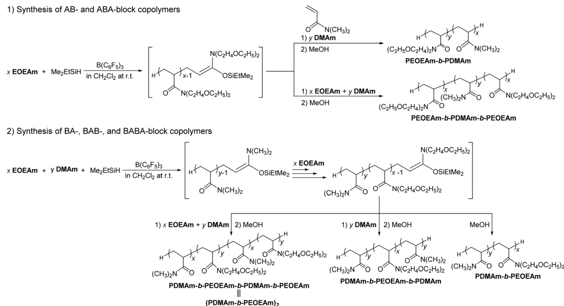
Scheme 2 Synthesis of (1) PEOEAm- b -PDMAm and PEOEAm- b -PDMAm- b -PEOEAm and (2) PDMAm- b -PEOEAm, PDMAm- b -PEOEAm- b -PDMAm, and (PDMAm- b -PEOEAm) 2 by the block and random GTcOP of EOEAm and DMAm.
