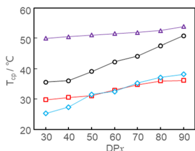
Fig. 5 Dependence of T_{cp} on DP_x for PDEAm x -OH (Δ), PDEAm x -b-PCL y (○), PDEAm x -b-PTMC y (□), and PDEAm x -b-PLLA y (◇).
