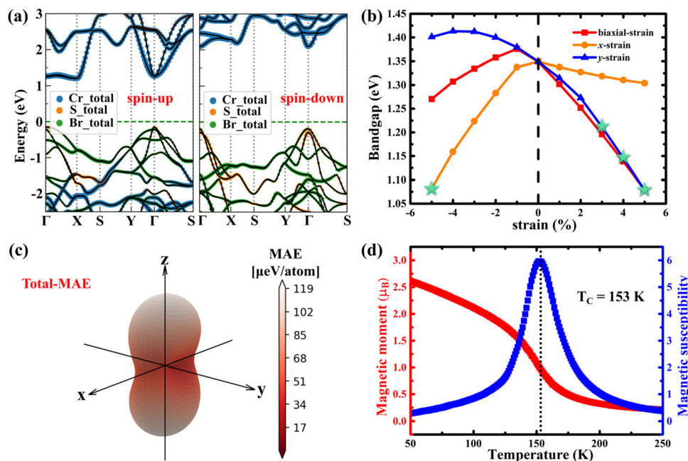
Fig. 2 (a) The band structure of the CrSBBr monolayer. (b) The band gaps of the CrSBBr monolayer under biaxial and uniaxial strains (−5%–5%). The star represents a direct band gap. (c) Angular dependence of the total-MAE of the CrSBBr monolayer with the direction of magnetization lying on the whole space. (d) The magnetic moment and magnetic susceptibility as functions of temperature for the CrSBBr monolayer.
