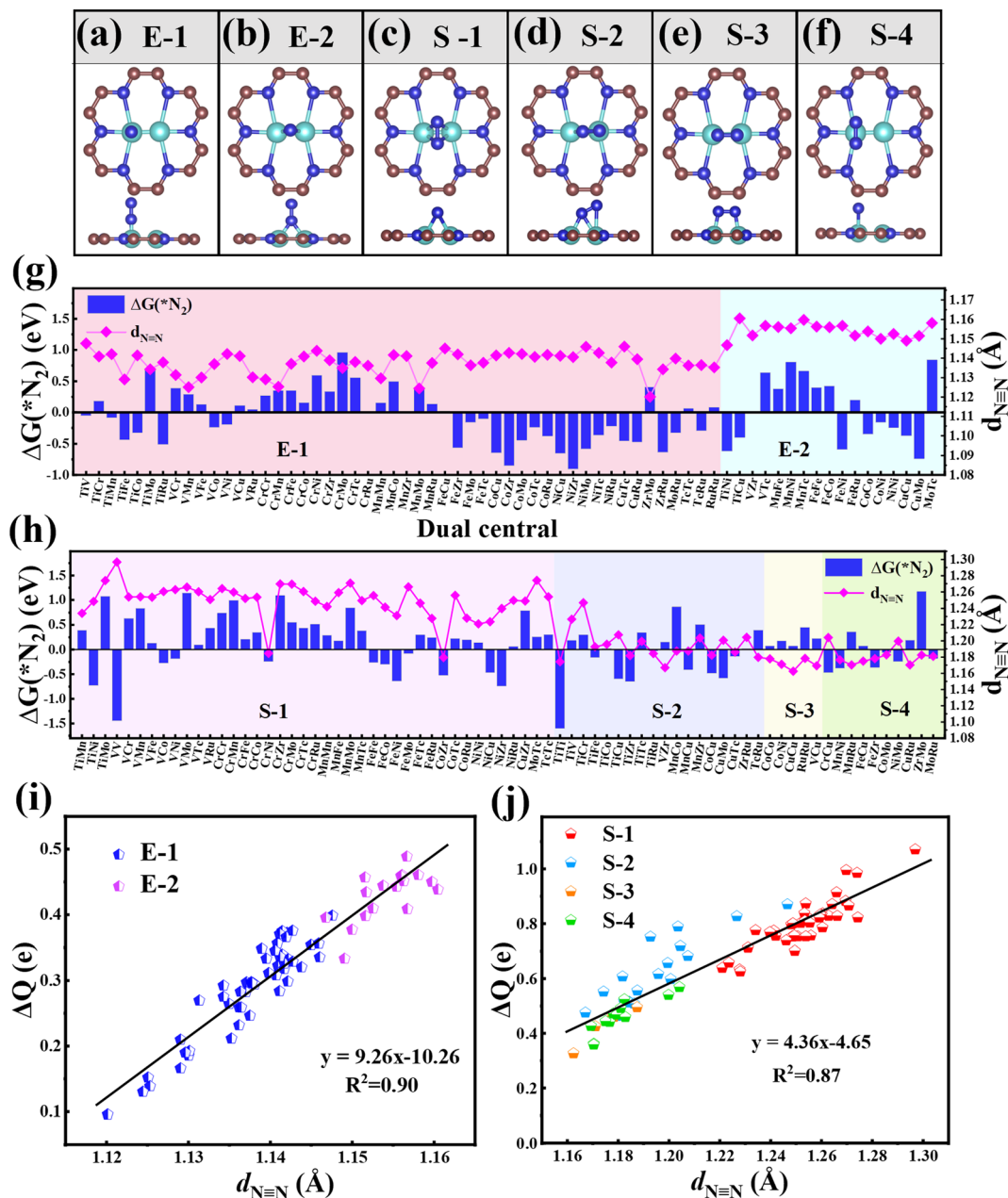
Fig. 2 The considered adsorption configurations of (a and b) end-on (E-1, E-2) and (c–f) side-on (S-1, S-2, S-3, and S-4) for N_2 on the \text{TM}_1\text{TM}_2@C_9N_4 substrate. Gibbs free energy change G(*N_2) values and N \equiv N bond lengths of *N_2 ( d_{N \equiv N} ) adsorbed on 77 \text{TM}_1\text{TM}_2@C_9N_4 catalysts with (g) end-on and (h) side-on adsorption configurations. Relationships between charge transfer ( \Delta Q ) and d_{N \equiv N} adsorbed on 77 \text{TM}_1\text{TM}_2@C_9N_4 catalysts through (i) end-on and (j) side-on adsorption configurations.
