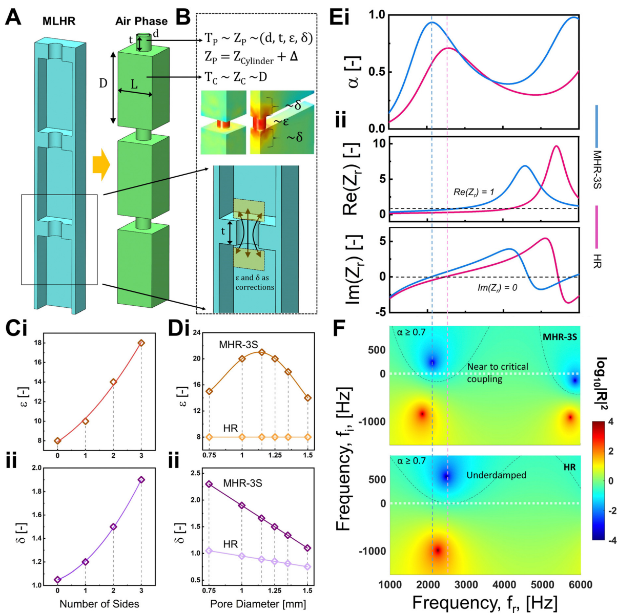
Fig. 5 Analytical model and acoustic impedance of the HR and MHR. (A) A schematic of the multi-layered HR and its inner air phase. (B) A schematic illustration of the acoustic impedance and transfer matrix of the pore and cavity, and the end correction factors. The (C(i)) resistance and (ii) reactance end correction factors of HR with 0 sides to MHR with 1 to 3 sides. The (D(i)) resistance and (ii) reactance end correction factors of HR and MHR-3S with varying pore diameters. The analytically calculated (E(i)) sound absorption coefficient curves, the (E(ii)) curves of the real and imaginary parts of Z_r , and the (F) complex plane diagrams of the MHR-3S and HR.
