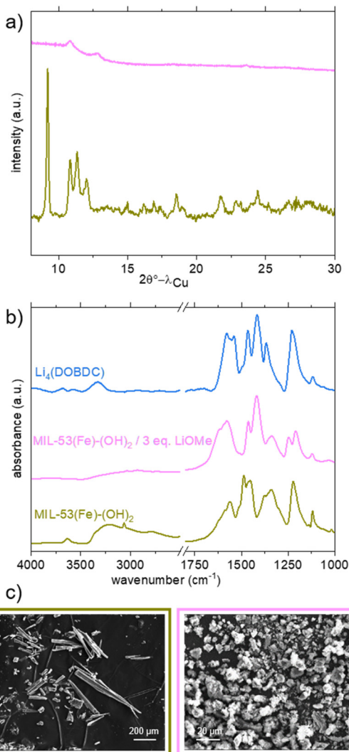
Fig. 5 Characterisation of \text{MIL-53(Fe)-(OH)}_2 and its lithiated product from LiOMe in MeOH/THF. a) PXRD patterns ( \lambda = 1.5406 Å); b) IR spectra; c) SEM pictures. Data related to dry \text{MIL-53(Fe)-(OH)}_2 , \text{Li}_4(\text{DOBDC}) and the lithiation product are shown in khaki, blue and pink, respectively.
