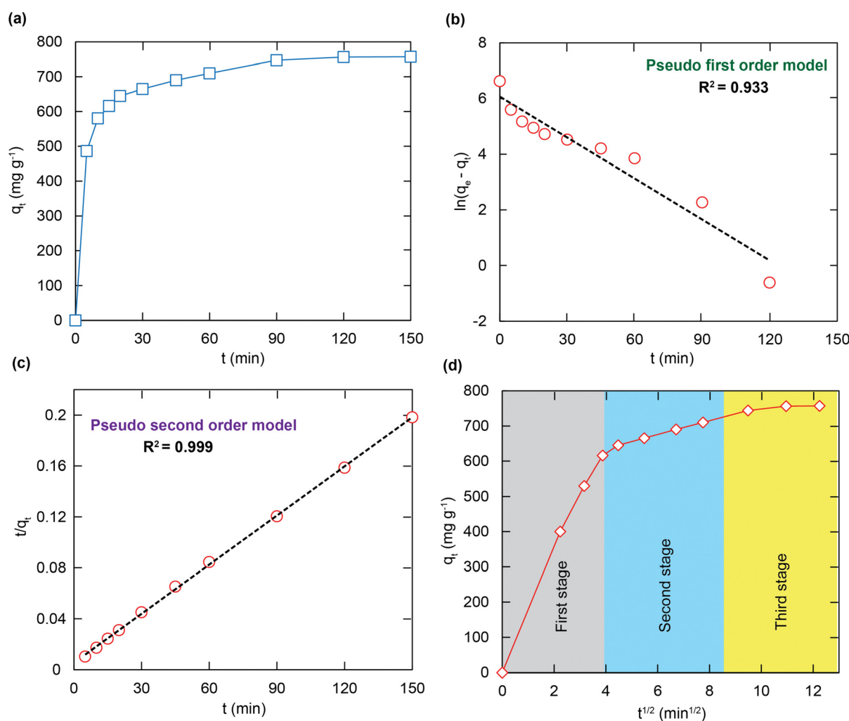
Fig. 6 The kinetic curve for the adsorption of RhB onto \text{H}^+ \subset \text{BUT-8}(\text{Cr}) [ m = 10 \text{ mg} , V_{\text{RhB}} = 100 \text{ mL} , C_o = 100 \text{ mg L}^{-1} , \text{pH} = 3 ] (a); data fitting with the adsorption kinetic models: pseudo first order (b), pseudo second order (c) and intra-particle diffusion model (d).
