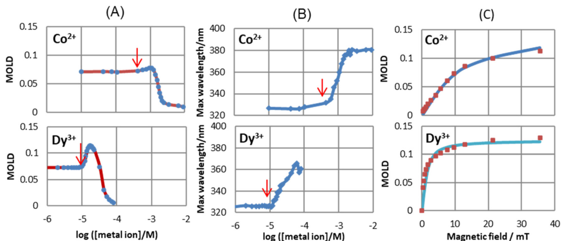
Fig. 14 Effect of metal ion concentrations of Co^{2+} and Dy^{3+} on (A) max. MOLD values and (B) max. wavelength of MOLD spectra (35.6 mT). The red arrows show the critical association concentrations. (C) Langevin analysis in [Co^{2+}] = 9.24 \times 10^{-4} M and [Dy^{3+}] = 1.67 \times 10^{-5} M, 0.00165 wt% MNPs. Reproduced with permission from ref. 205. Copyright © 2020, the American Chemical Society.
