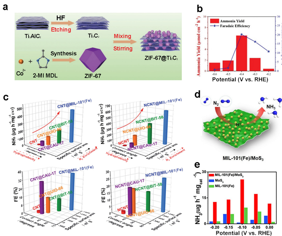
Fig. 13 MOF-based NRR electrocatalysts. (a) Schematic diagram of the synthesis of the \text{ZIF-67@Ti}_3\text{C}_2 composite; (b) \text{NH}_3 yield and faradaic efficiency of the \text{ZIF-67@Ti}_3\text{C}_2 composite at each given potential. Reproduced with permission. 111 Copyright 2021, The Royal Society of Chemistry; (c) optimal catalytic results of NRR catalysts obtained by adjusting the water contact angle and specific surface area. Reproduced with permission. 109 Copyright 2021, The Royal Society of Chemistry; (d) schematic diagram of the NRR process of \text{MIL-101(Fe)/MoS}_3 ; (e) comparison of the \text{NH}_3 yield of \text{MIL-101(Fe)/MoS}_3 , \text{MoS}_3 and \text{MIL-101(Fe)} at each given potential. Reproduced with permission. 110 Copyright 2022, Springer Nature.
