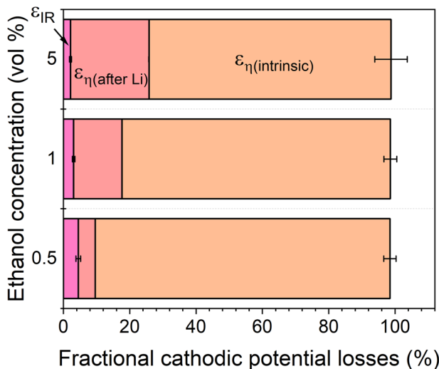
Fig. 4 A plot to show the fractional potential losses in the cathodic reaction for the lithium-mediated nitrogen reduction system due to overpotential and ohmic losses for a 0.6 M \text{LiClO}_4 in THF electrolyte with varying ethanol content. Fractional energy losses obtained using eqn (18) and (19).
